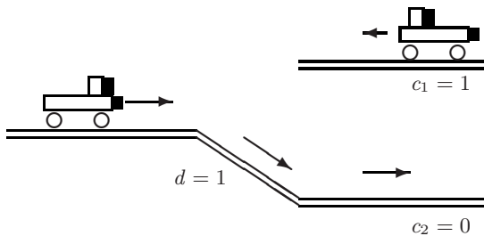
Fig. 4. Railway points: The situation that is tested by MC/DC (normal operation)
