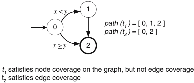
Fig. 4. A graph showing Node and Edge Coverage
