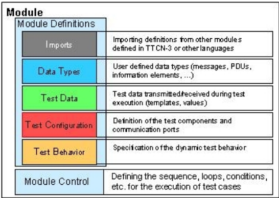
Fig. 2. The TTCN-3 Module Structure
