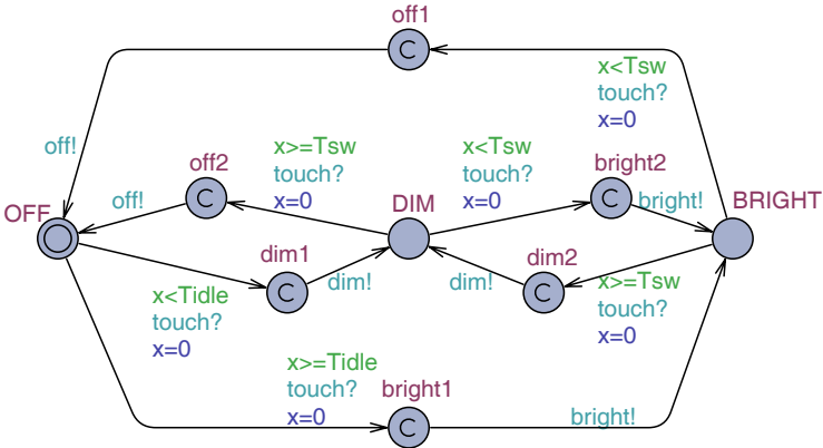
Fig. 3. Light Controller
