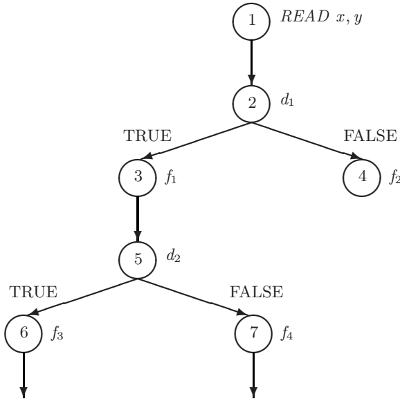
Fig. 2. Flow graph of a program fragment
