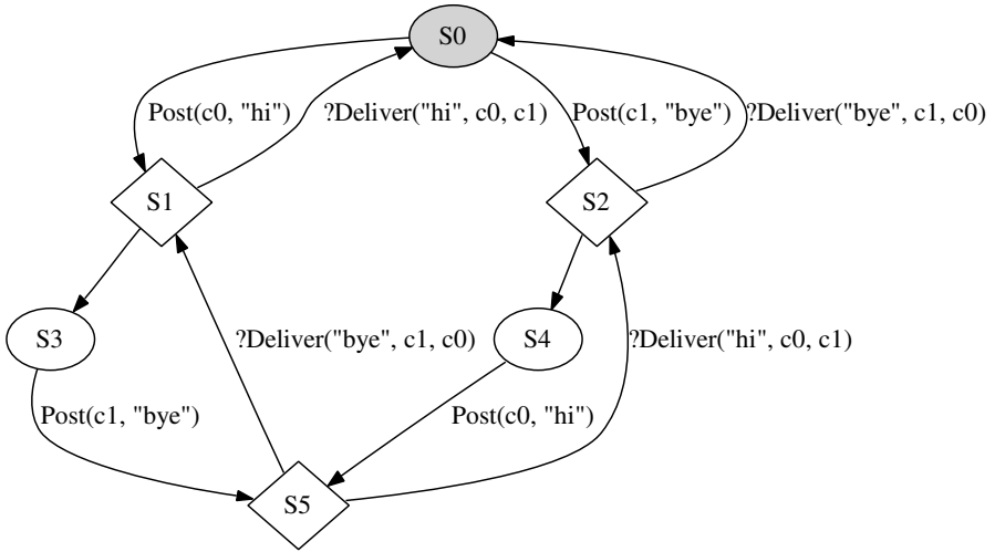
Fig. 4. Exploration of the Chat model with two clients ( c0 and c1 ), a fixed message (“hi” sent by c0 and “bye” sent by c1 ) and the restriction that the number of pending deliveries for each client is at most 1. The initial state is shown in grey. Action labels prefixed by “?” indicate observable actions. Labels without prefix indicate controllable actions. Active states are shown as ovals. Passive states are shown as diamonds. The unlabeled transitions represent an internal transition (“timeout”) from passive to active.
